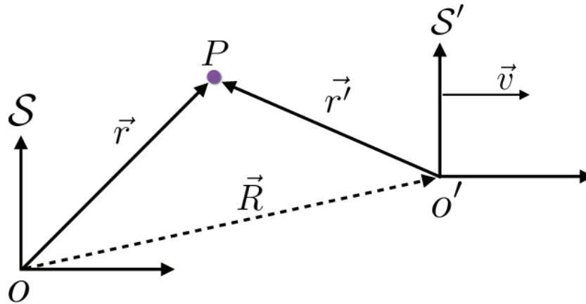
Figure 1. Two inertial systems S and S' moving relative to each other with velocity \vec{v} . Position vector of a point P in S is \vec{r} \equiv (x, y, z, t) \equiv x_\mu and that in S' is r' \equiv (x', y', z', t') \equiv x'_\nu .
