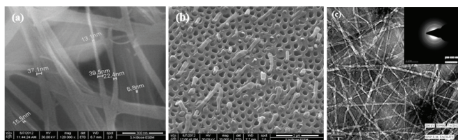
Fig. 1. (a) SEM showing bundles of nanorod, (b) SEM of nanorod protruding from pores and (c) TEM of BFO nanorods and corresponding SAED pattern shown in the inset.
