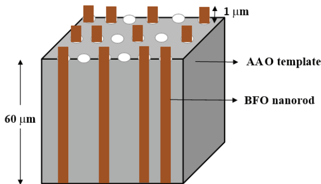
Fig. 4. Schematic diagram of BFO nanorod developed on AAO template. 1 \mu m protrusion from the pores is there with the depth of the pores being 60 \mu m.
