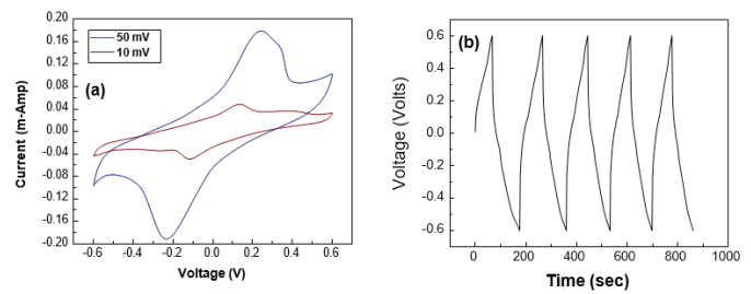
Fig. 2. (a) Cyclic voltammogram of BFO on AAO at different scan rates and (b) Charge-discharge cycle of BFO on AAO template at 30μAmp current.
