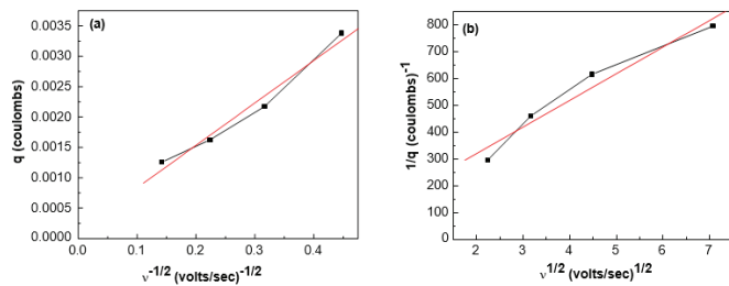
Fig. 3. (a) q^* versus v^{-1/2} plot to extract q_{out} (b) 1/q^* vs. v^{1/2} to extract q_{tot}^* .
